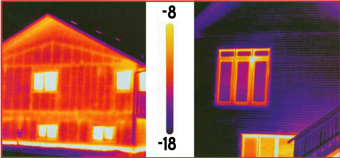
Thermal image of a conventionally built home showing heat loss across the entire wall.
